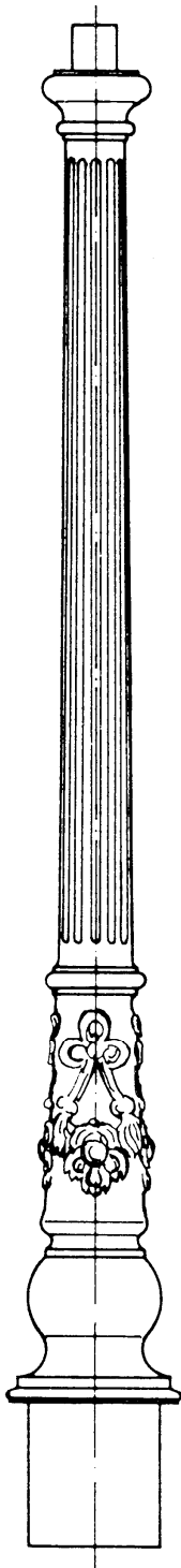
THK-685 Candelabra top with Spigot \varnothing 60 mm or flanged connections Weight: 82 kg
